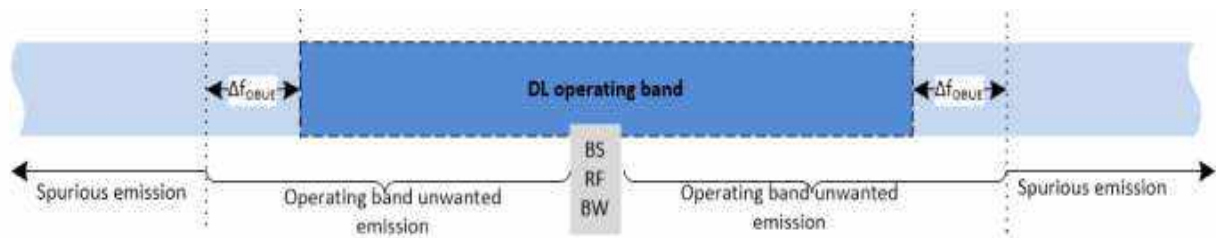
Gambar 5. Unwanted Emission
