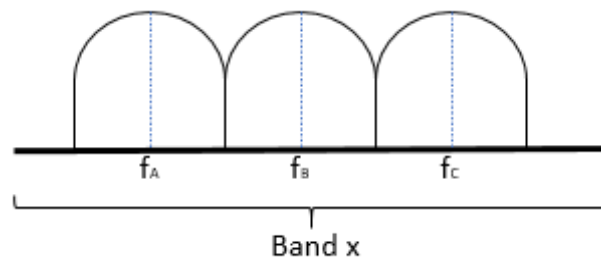
Gambar 1. Intraband contiguous .
